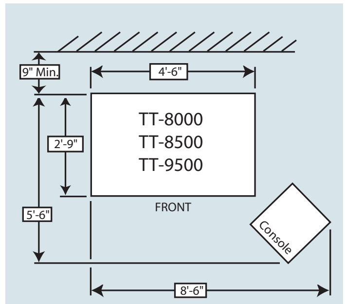
Floor Layout
